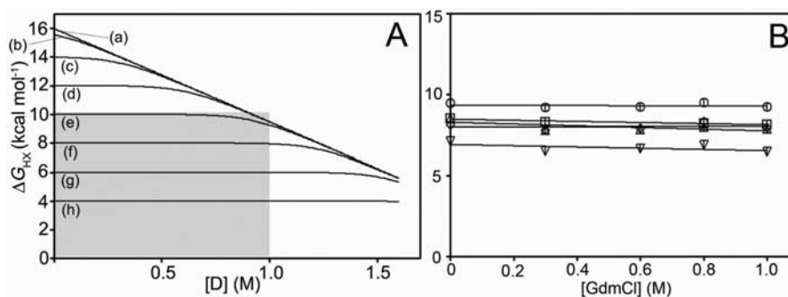
Figure 2. Comparison of calculated and observed exchange energies. (A) Estimation of \Delta G_{HX} versus denaturant concentration for different exchange mechanisms. All curves are generated by Eq. (1), with m=6.5 kcal mol -1 M -1 , \Delta G_{HX}^0=16 kcal mol -1 , and T=310 K. Lines (a)–(h) are generated using different values of \Delta G_{pt} from 16 to 4 kcal mol -1 . (B) Measurable H/D exchange peaks at pH 7.4, 37 °C as a function of denaturant concentration. Only residues on \beta -strand 1 are shown, the rest are shown in supplementary material. V12 (squares), L18 (triangles), D19 (reverse triangles), G20 (diamonds), and D21 (circles).
